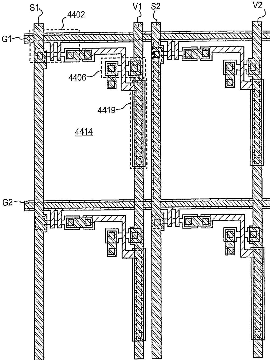
FIG. 41 PRIOR ART
